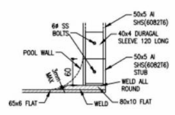
DETAIL FOR POST BASE SCALE 1 : 5
