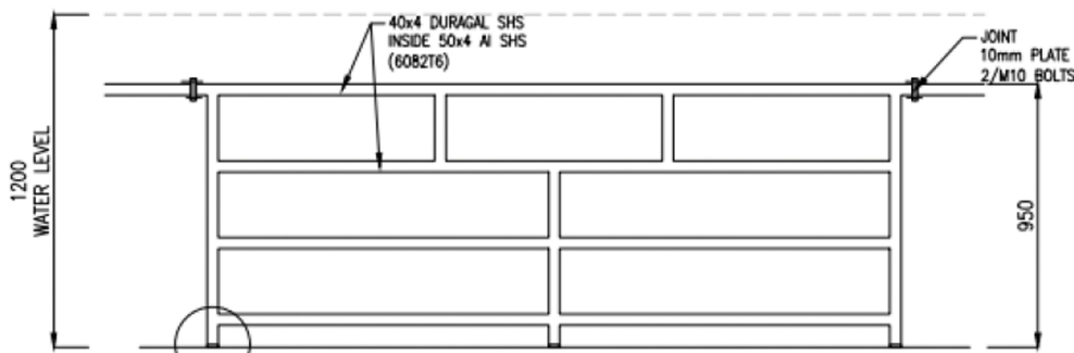
ELEVATION SCALE 1 : 20
