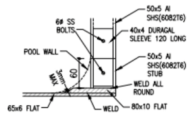
DETAIL FOR POST BASE SCALE 1 : 5
