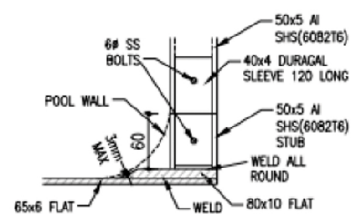
DETAIL FOR POST BASE SCALE 1 : 5
